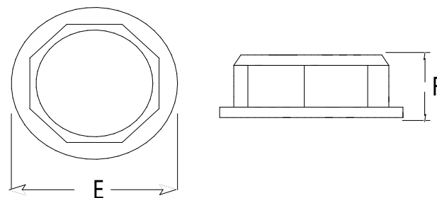
Cupsink Backnut
